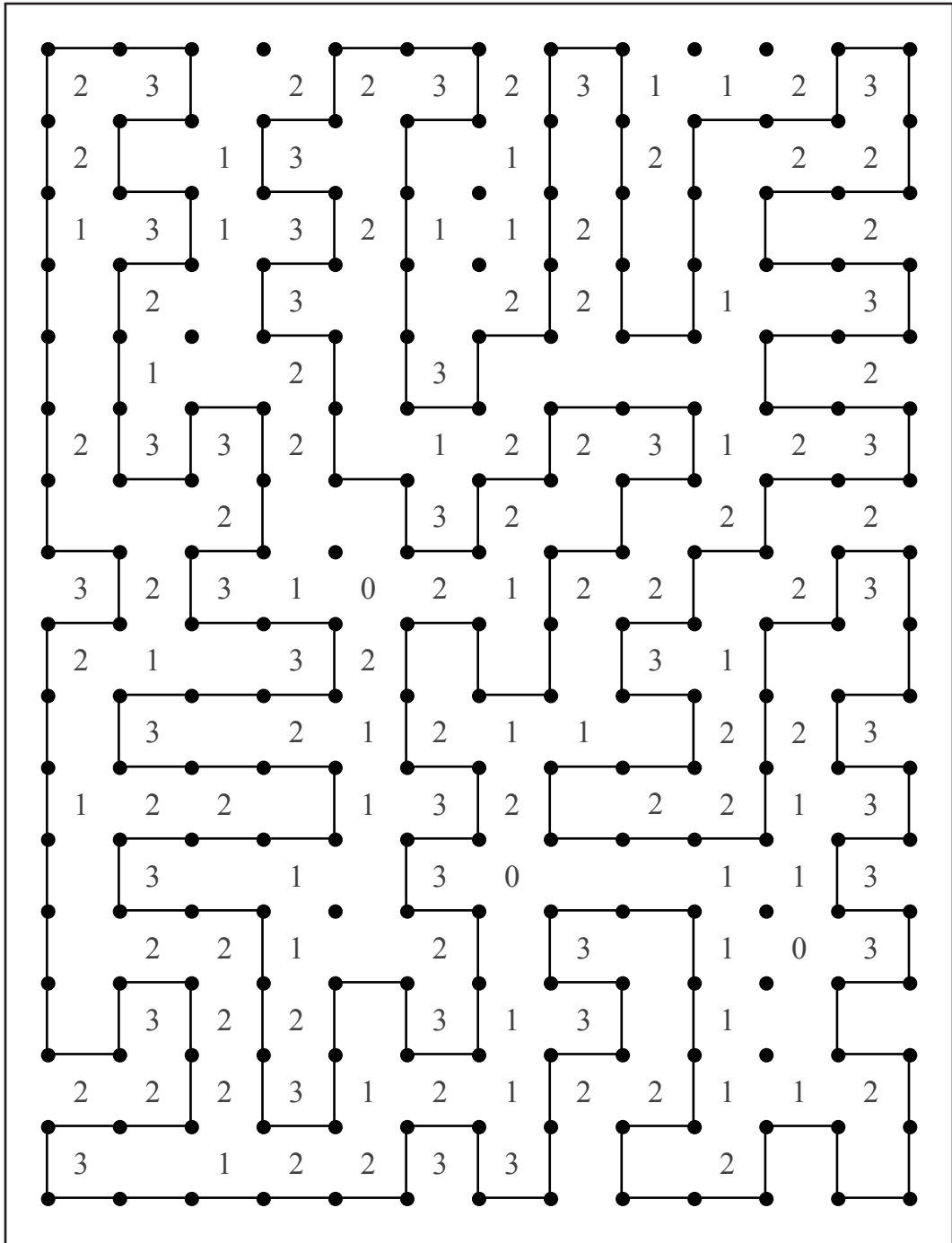
1216 SLITHERLINK EASY 15
