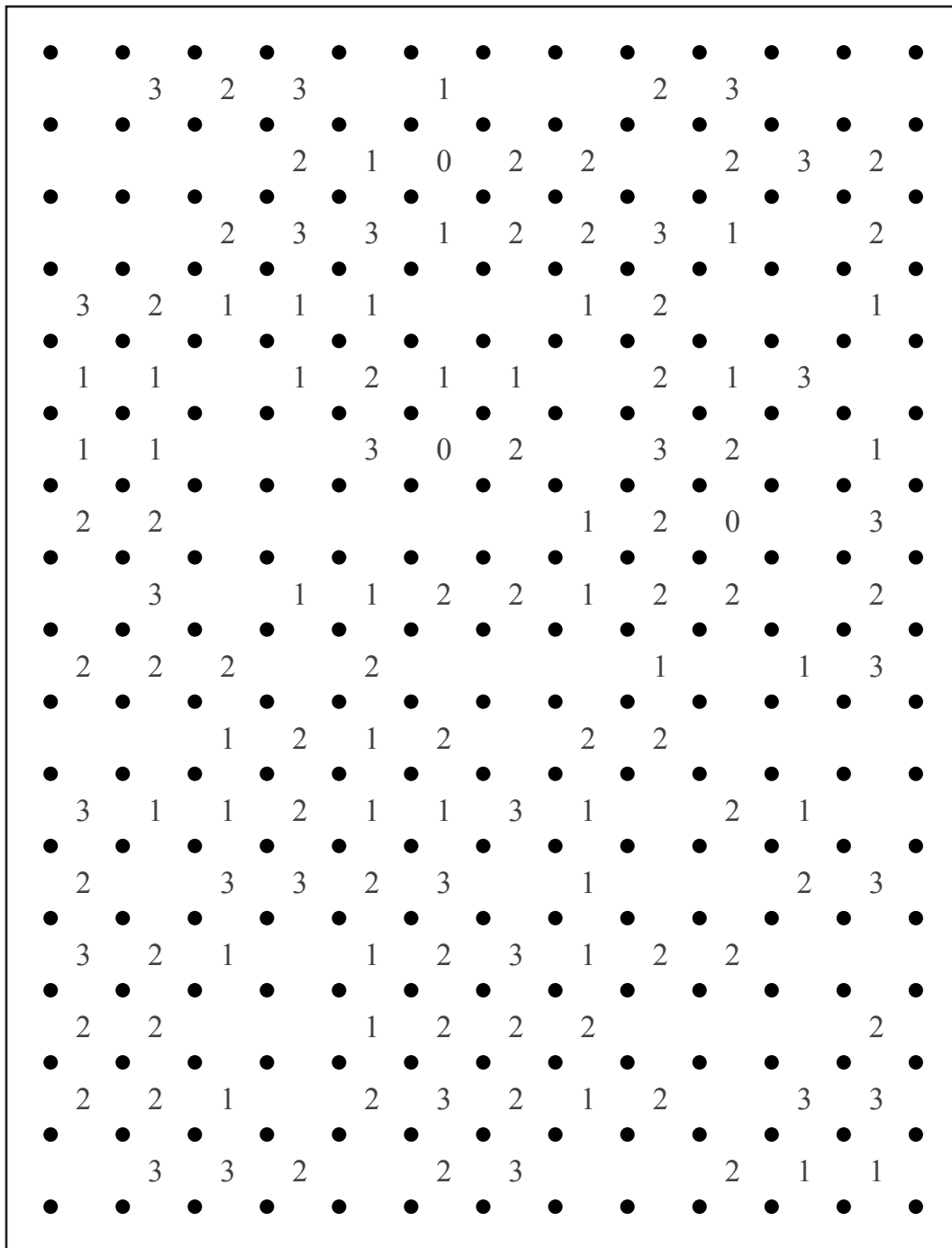
1216 SLITHERLINK EASY 10
