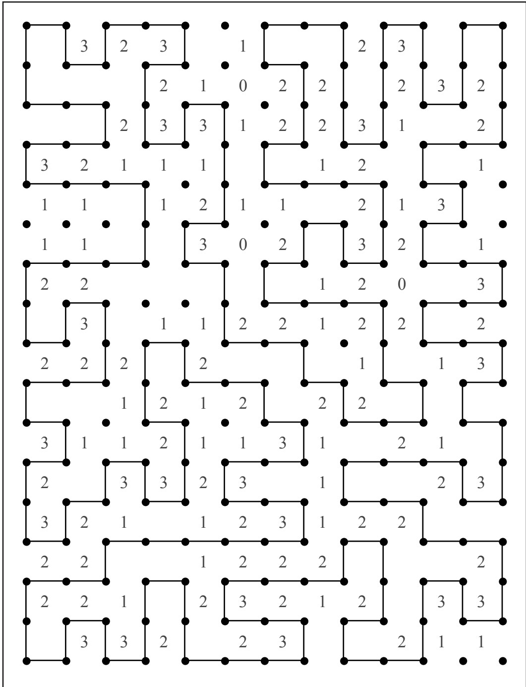
1216 SLITHERLINK EASY 10
