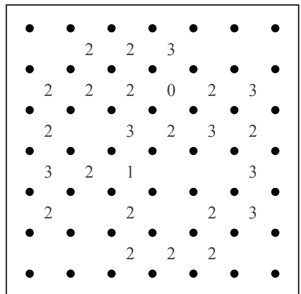
0606 SLITHERLINK EASY 24
