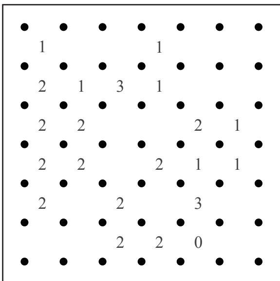
0606 SLITHERLINK EASY 23
