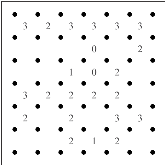
0606 SLITHERLINK EASY 21
