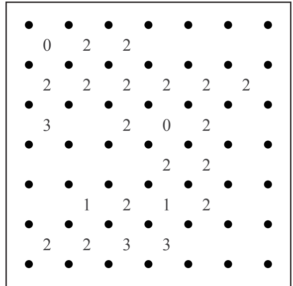
0606 SLITHERLINK EASY 22
